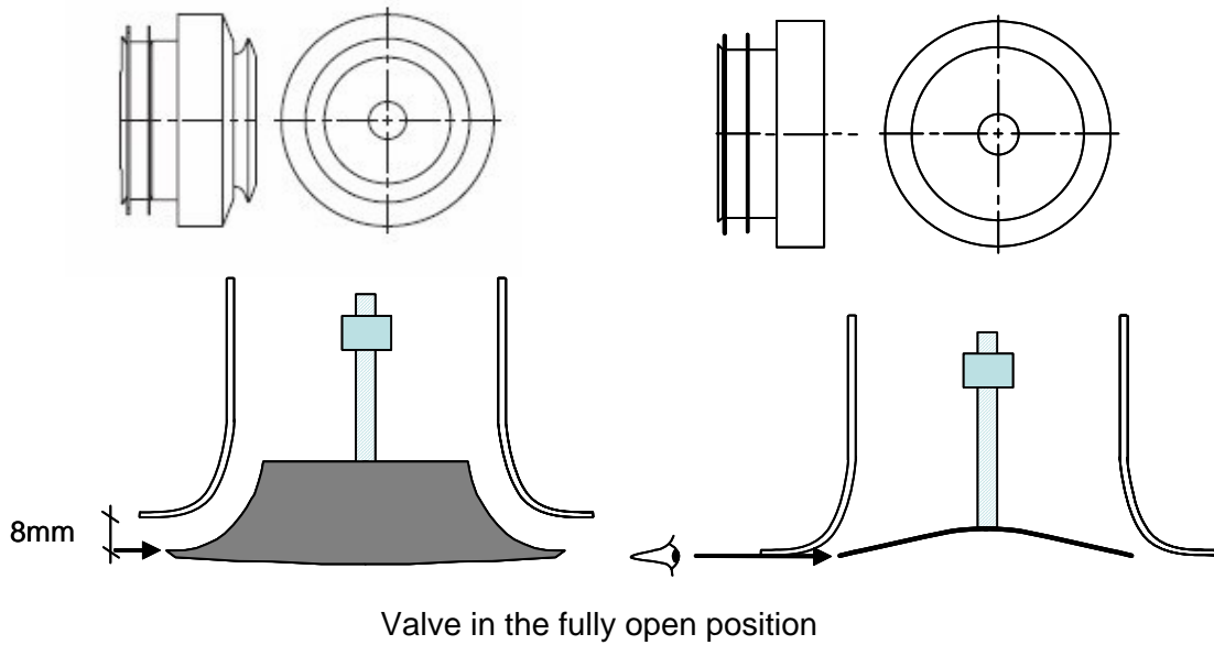
Figure 4 Examples of supply air terminal devices fully open
