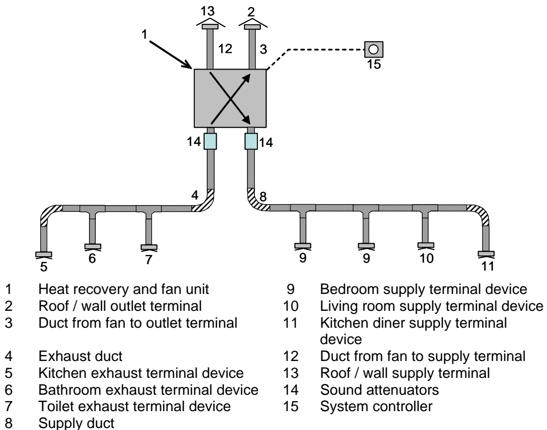
Figure 1 Typical components that may form part of a mechanical supply and exhaust ventilation system package with heat recovery
