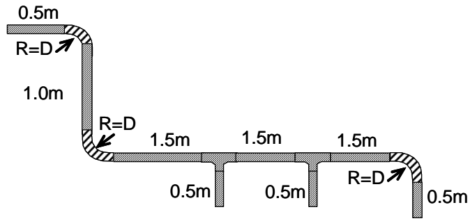
Long branched duct, 3 terminals
