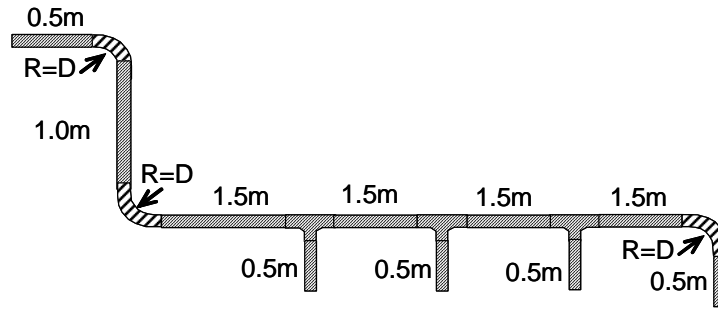
Long branched duct, 4 terminals
