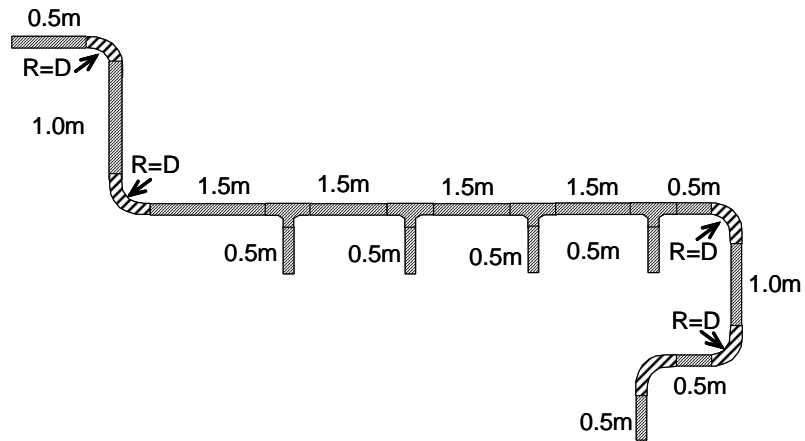
Long branched duct, 5 terminals
