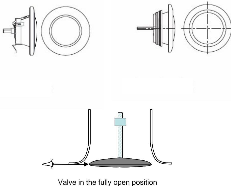
Figure 3 Examples of exhaust air terminal devices fully open
