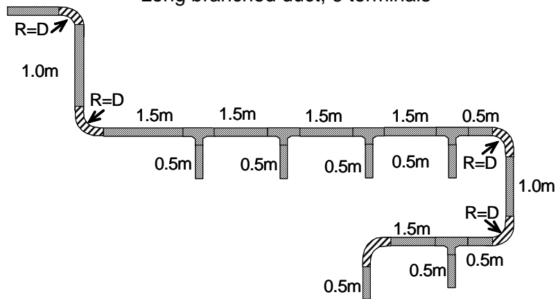
Figure 2 Examples of duct connections
